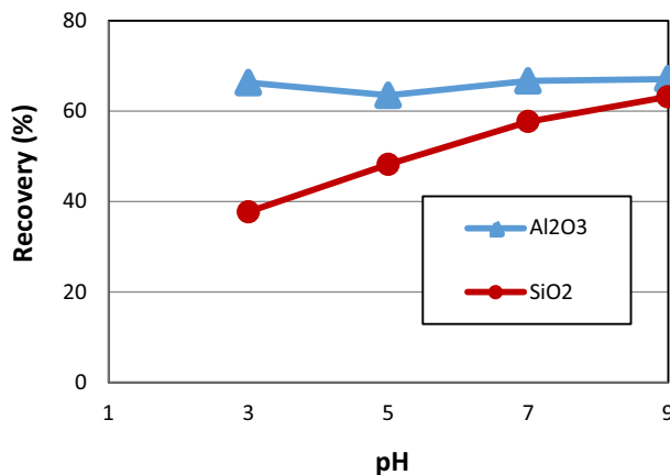
Figure 9. Flotation recovery of \text{Al}_2\text{O}_3 and \text{SiO}_2 as a function of pH with DDA as a collector (DDA 600 g/t, aluminum chloride 300 g/t, desliming -38 \mu\text{m} ).
